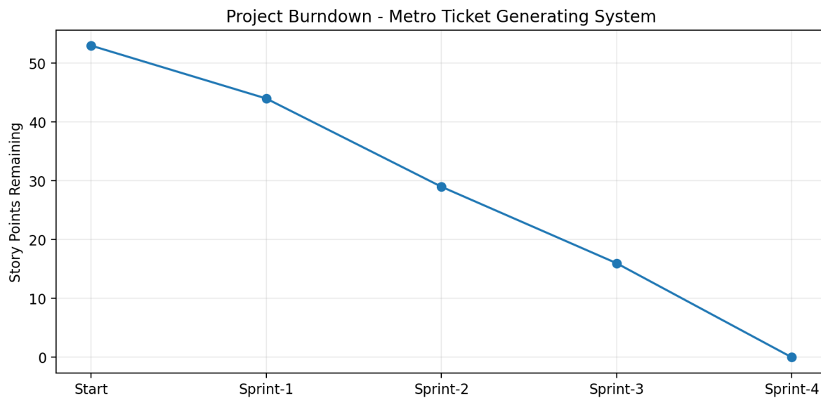
Figure 4. Project burndown based on the four-sprint planning model
